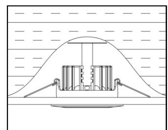
Fitting for Optional Insulation Spacer
