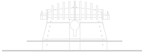
ECO16-23-31-HA3-MW Hole Adapter 170mm-285mm (two part adapter)
